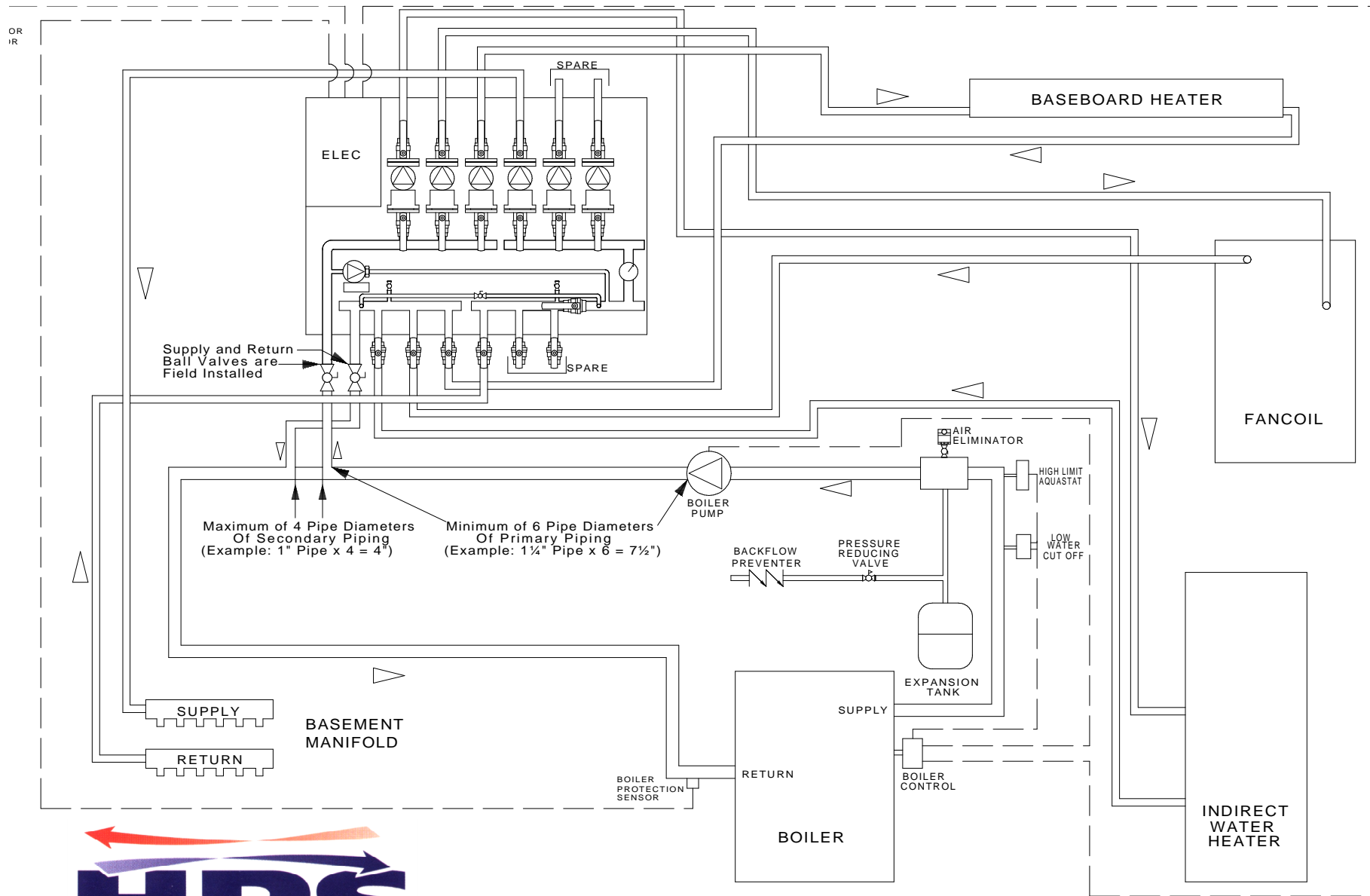
GENERIC HYDRONIC HEATING SCHEMATIC
