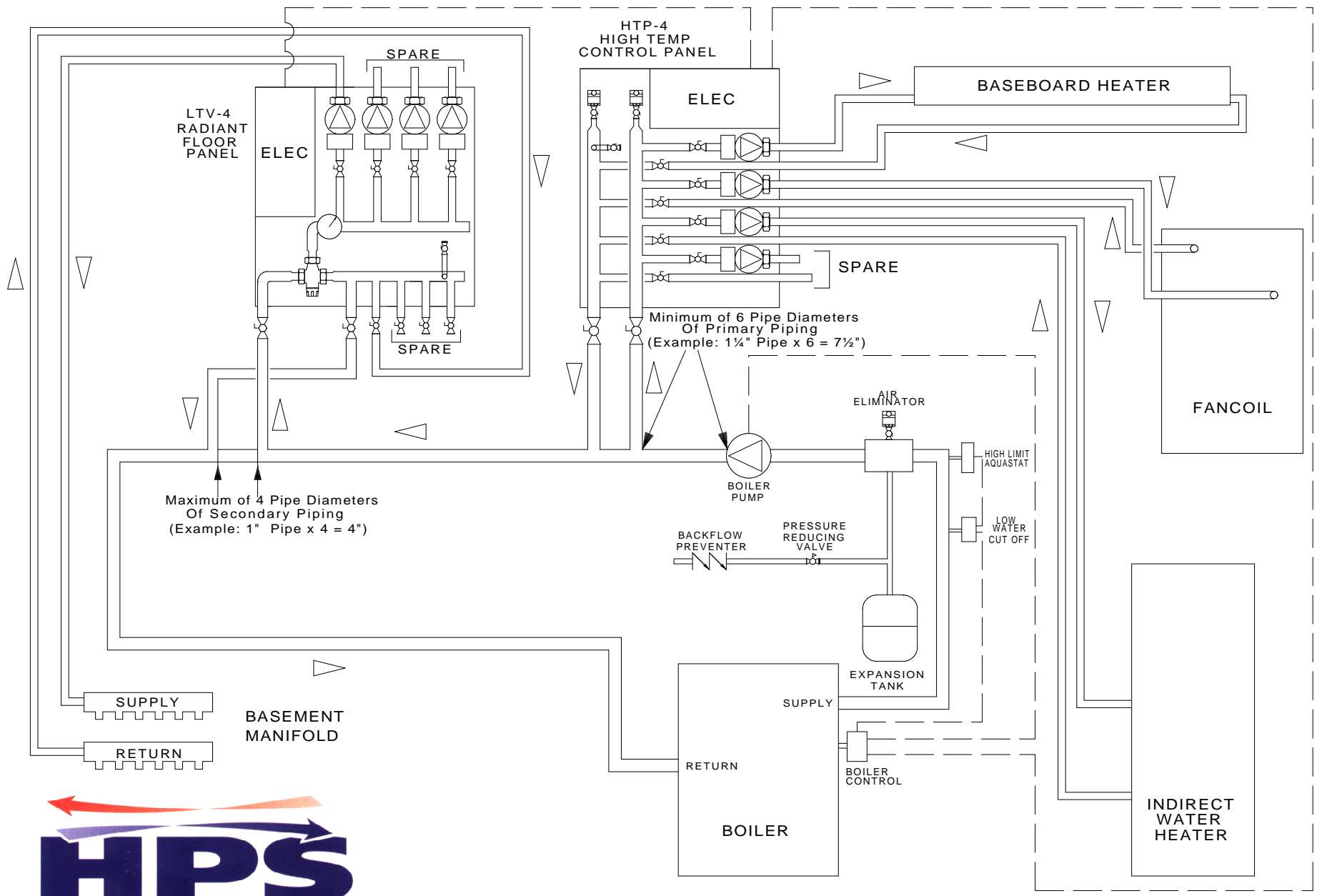
GENERIC HYDRONIC HEATING SCHEMATIC
